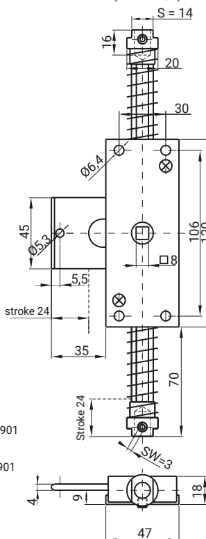
ZW8 (with hole \varnothing 8 )
