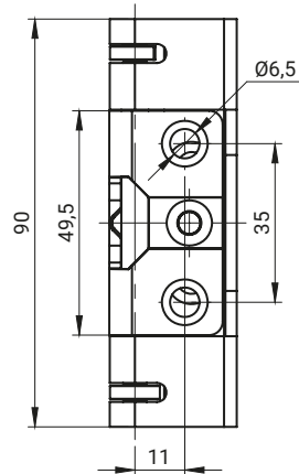
3.ST147.001
