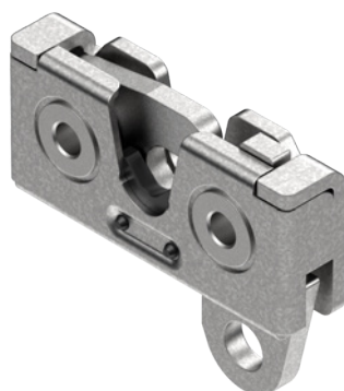
Lock 2.518.001 page 2A-119
