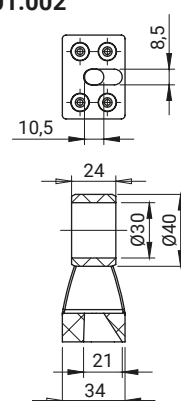
4.104.001.002
