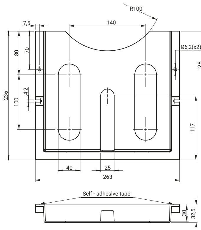
Pocket A4 4.420.001
