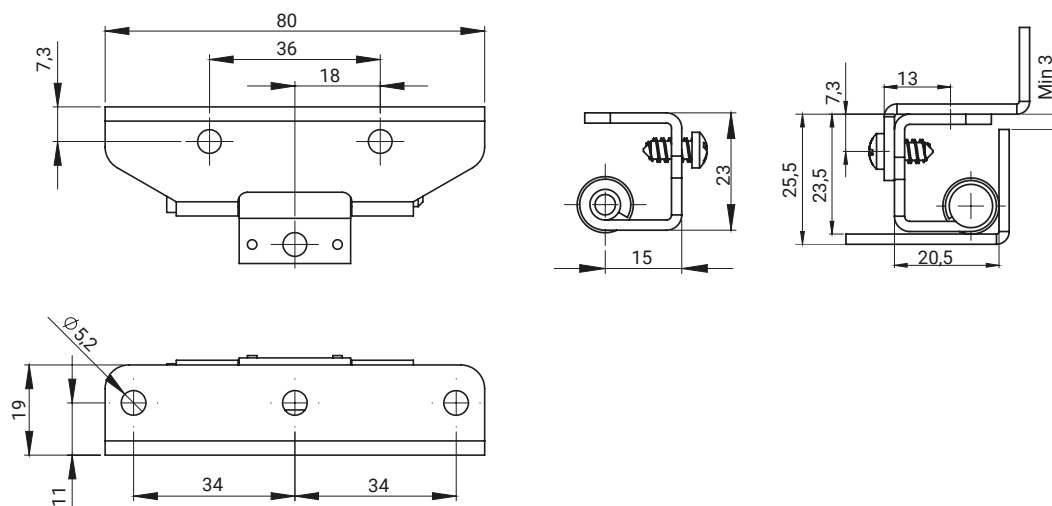
3.ST558 ver. 002
