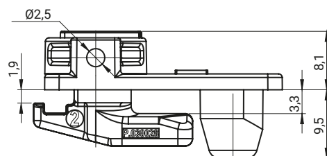
4.417.004
