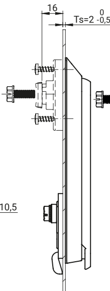
Version for a cap [N]
