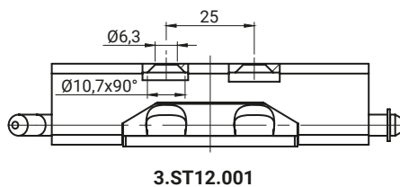
3.ST12.001
