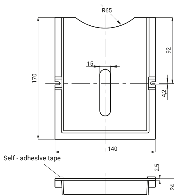
Pocket A6 4.420.002
