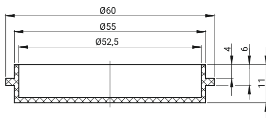
1C.916.003
