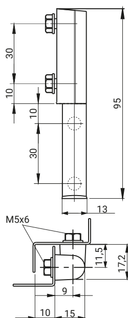
3.ZN151.001
