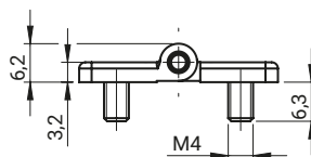
3.601.001
