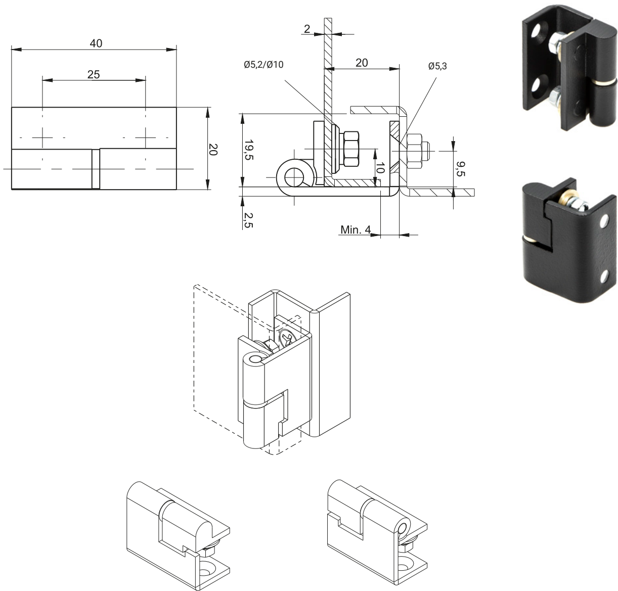
3.ZN140.001 RIGHT VERSION
