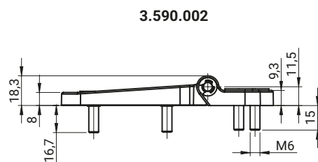
3.590.002
