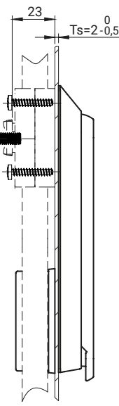
Version for a cogwheel mechanism [M]
