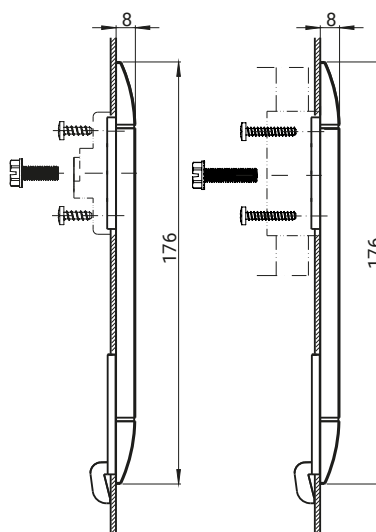
RW400.M RW410.M
