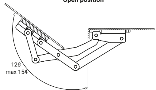
Open position
