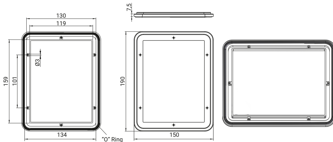
WINDOW 151 x 190
