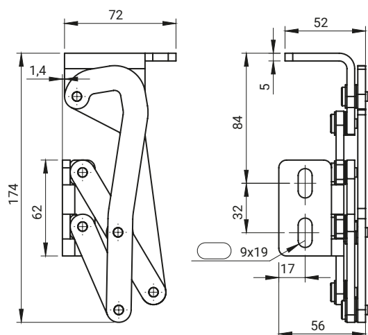
3.ST304.001
