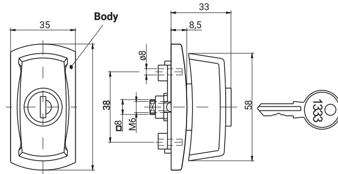
RW200.N ... (Used with Cap )
