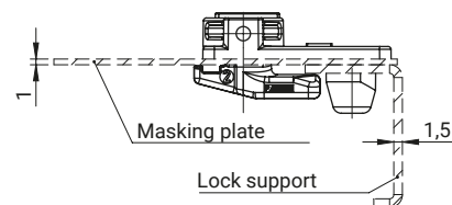
Auxiliary installation plan
