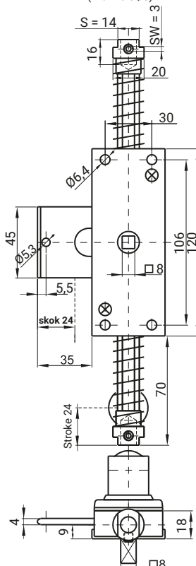
ZWP8 (with hole \varnothing 8 )
