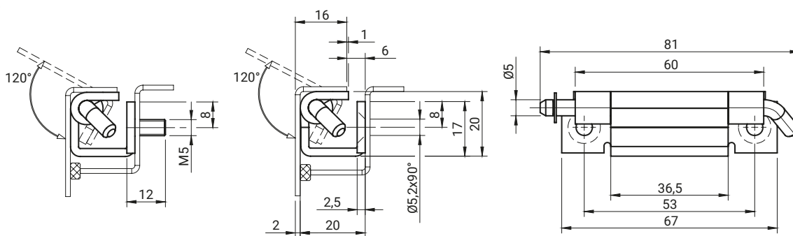
3.ST13.002
