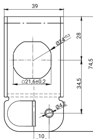
Blockade 2.904.102
