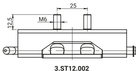
3.ST12.002
