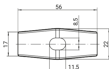
Bridge clamp 56 4.411.003
