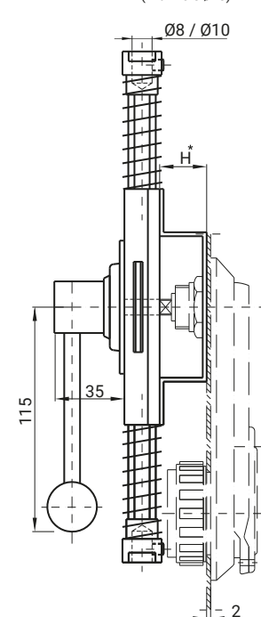
ZWP10 (with hole \varnothing 10 )
