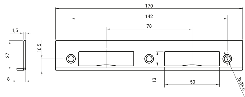
Latching element
