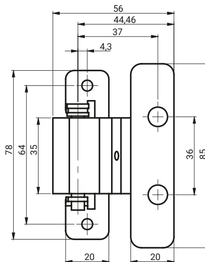
3.ST118.002
