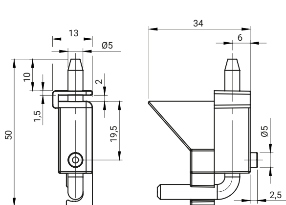
3.ST96.004
