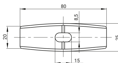
Bridge clamp 80 4.411.004
