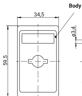
RW110.N ... (Used with Cap)
