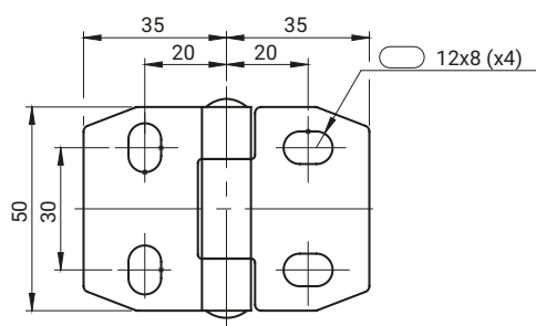
3.ST30.010
