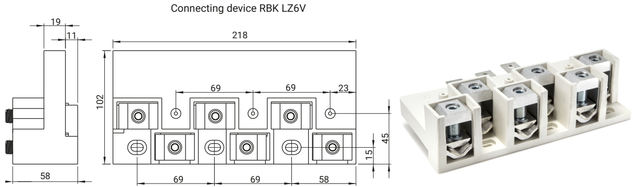
Terminals for connecting device 4.601.001
