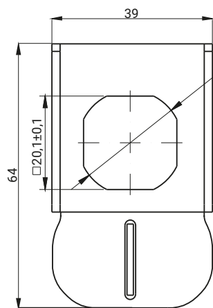
Blockade 2.902.001
