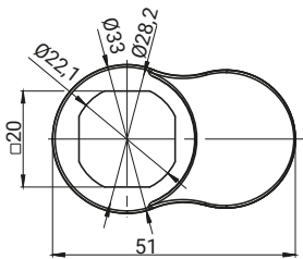
2.905.004A
