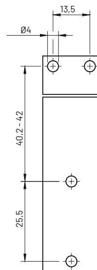
Mounting hole 3.562.002
