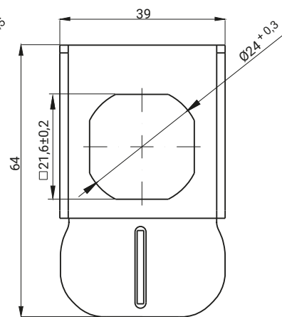
Blockade 2.902.002
