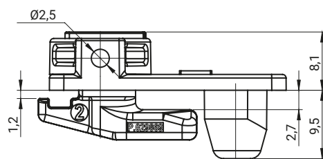
4.417.003
