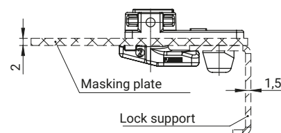
Auxiliary installation plan
