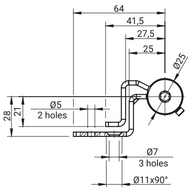
Closed position
