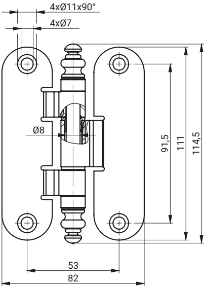
3.ST116.001
