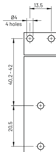
Mounting hole 3.562.001
