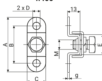
GROUND CLAMP 4.406
