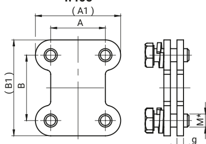
4-SCREW CLAMP 4.405
