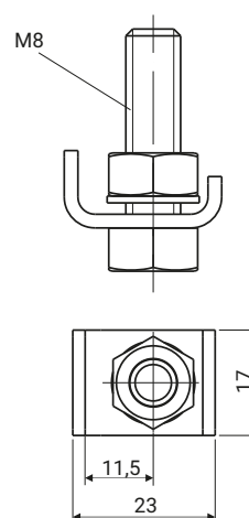
GROUND HOLDER 4.403.001
