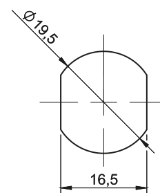
Mounting hole
