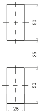
Mounting hole
