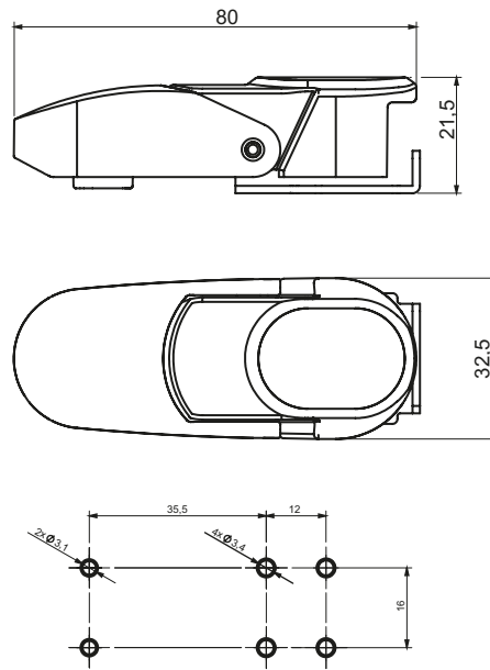
Mounting hole
