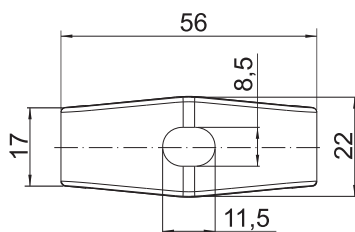
Bridge clamp 56 4.411.003
