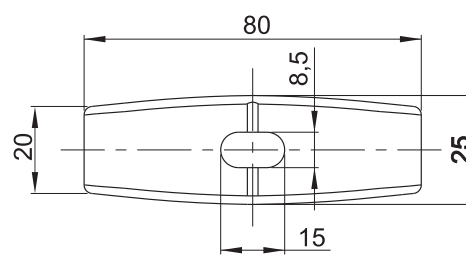
Bridge clamp 80 4.411.004
