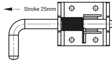
Open Position
