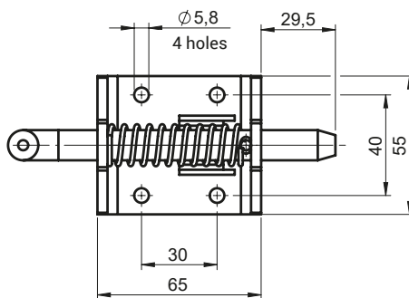
Locked Position
